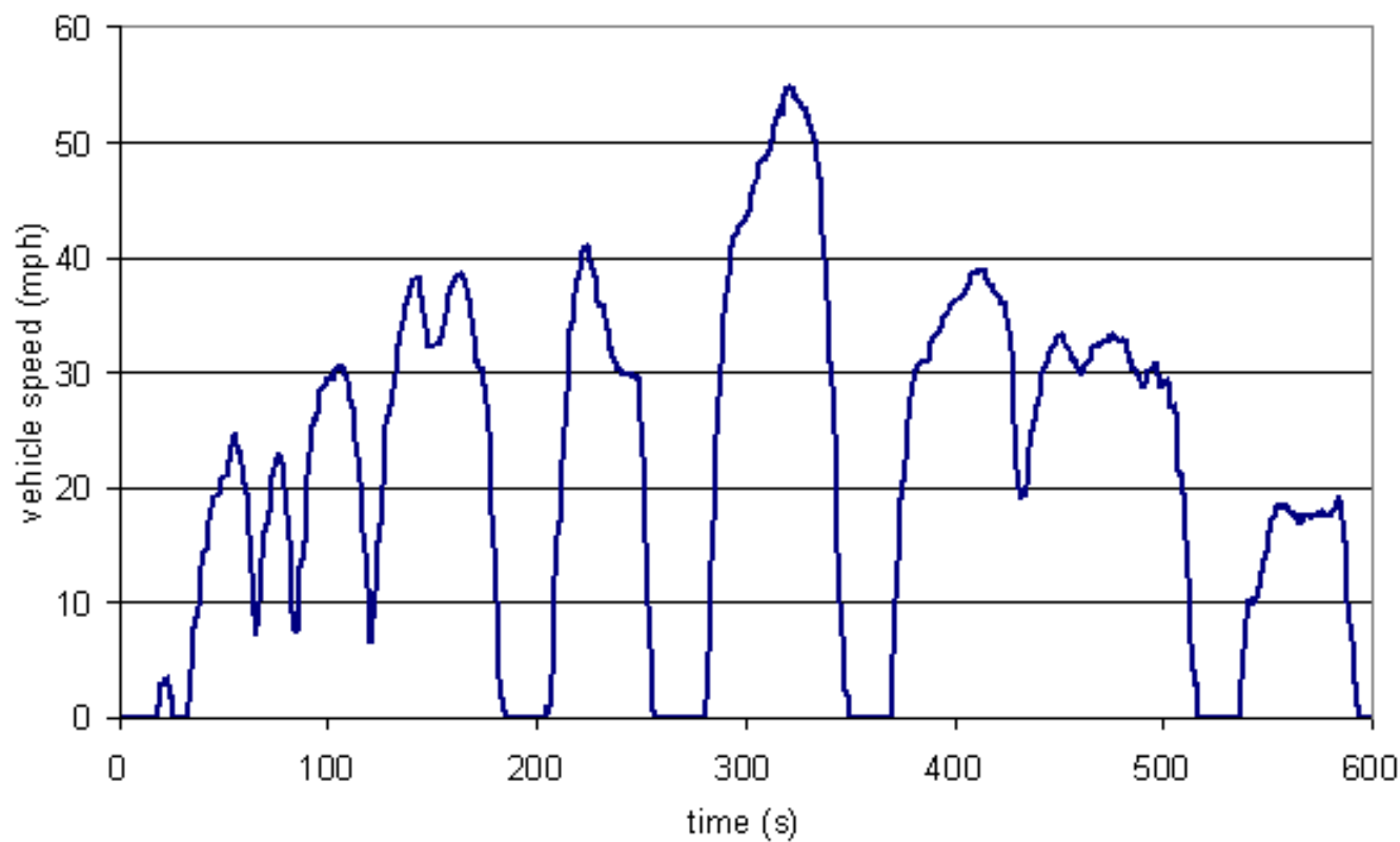
SC03 Driving Cycle
