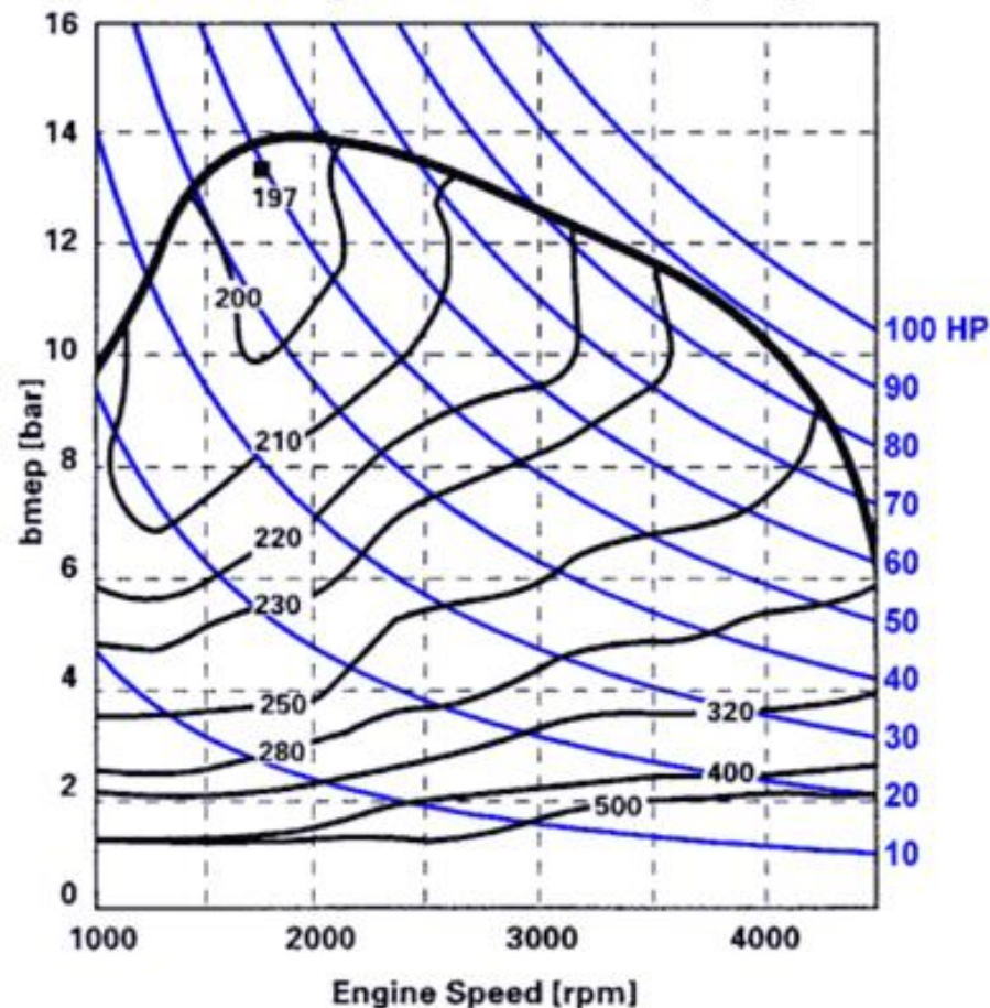
Fuel Consumption Map [g/kW-Hr]
