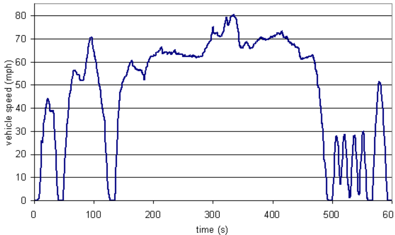
US06 Aggressive Driving Cycle
